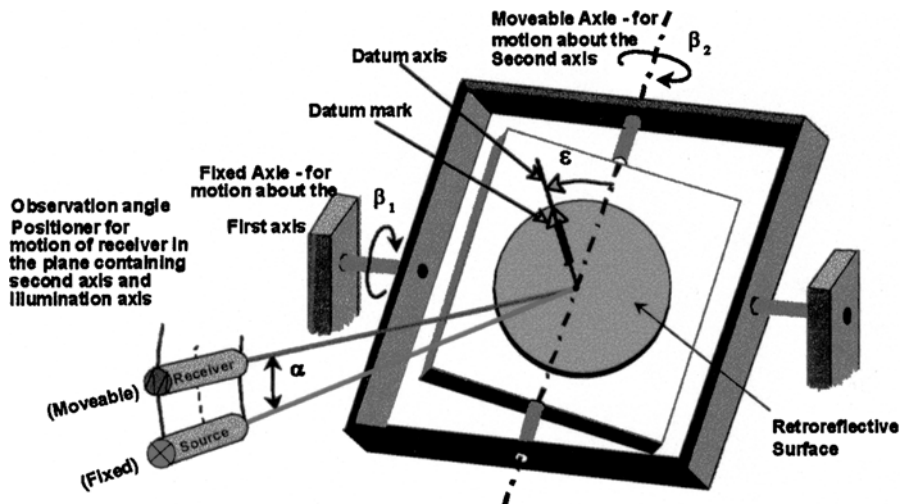
FIG. 2 View of Test Geometer for Measuring Retroreflection
